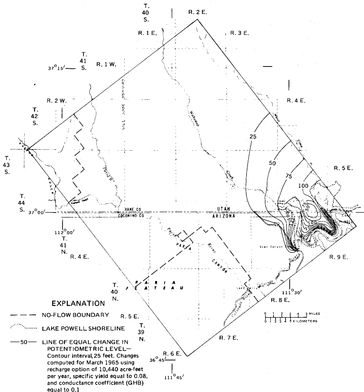
Figure 11.—Simulated changes in the potentiometric surface caused by 2 years of stress imposed on the system from Lake Powell.
