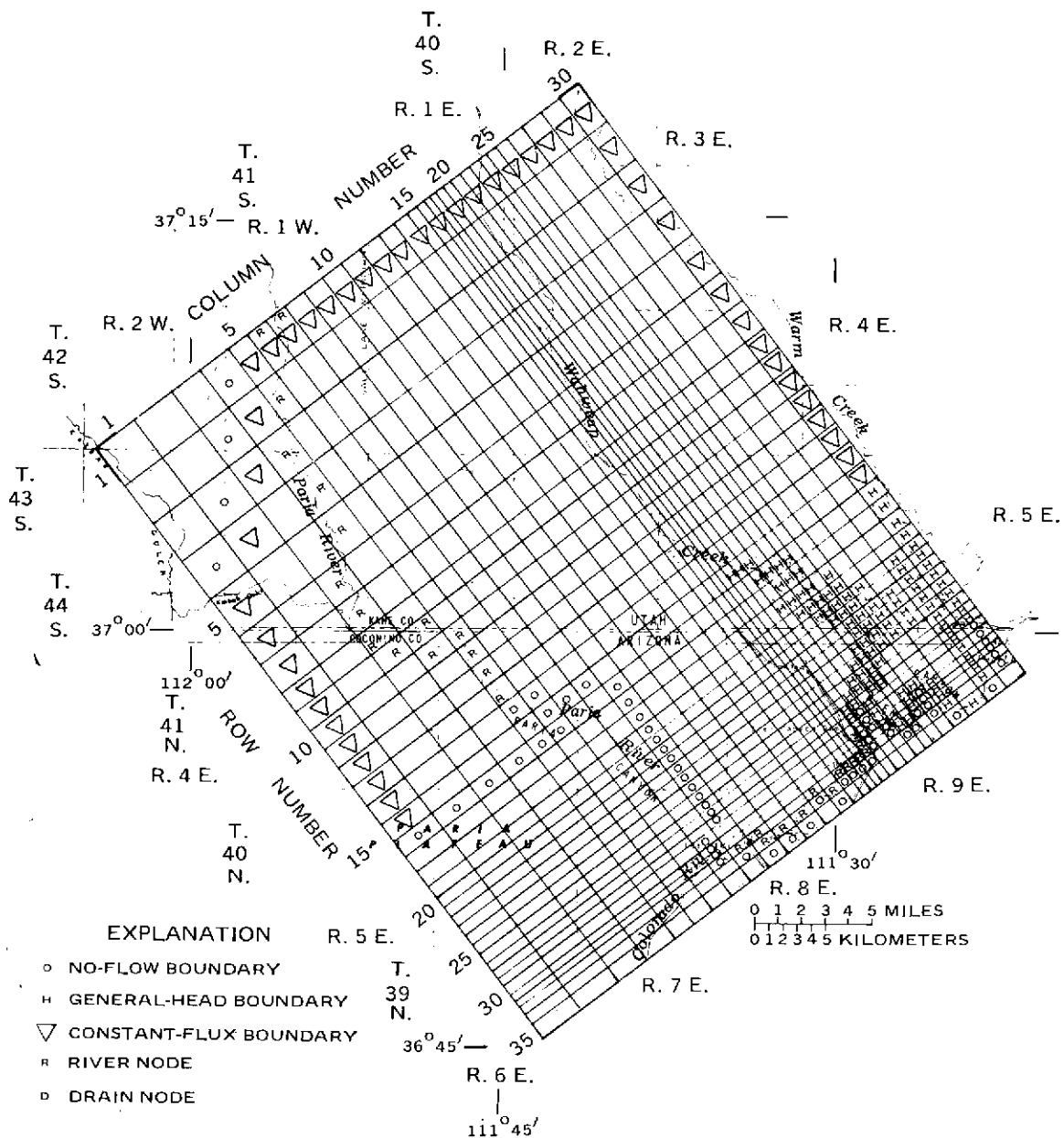
Figure 8.—Finite-difference grid and boundaries used in the transient-state model, 1983.
