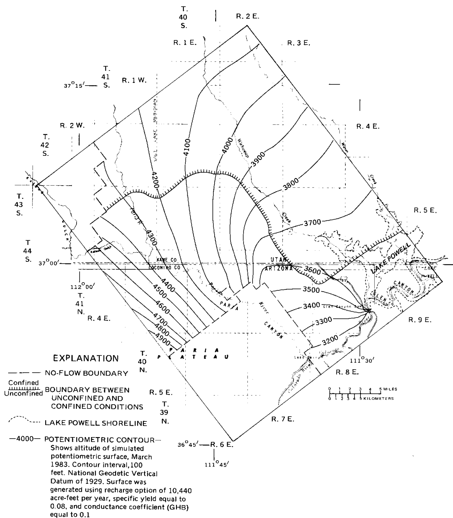
Figure 13.—Simulated potentiometric surface, March 1983.
