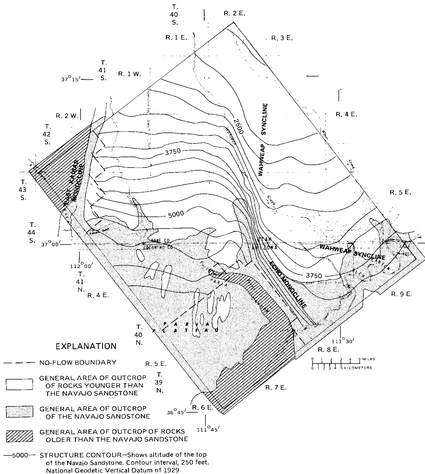
Figure 5.—Altitude of the top of the Navajo Sandstone and areas of outcrop.
